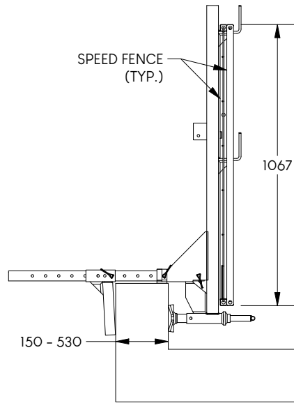
SPEED FENCE APPLICATION
