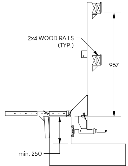
WOOD RAIL APPLICATION
