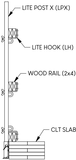
WOOD APPLICATION
