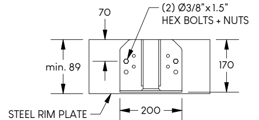
STEEL APPLICATION
