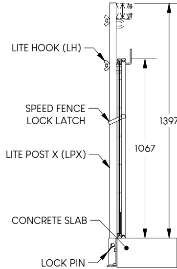
CONCRETE APPLICATION
