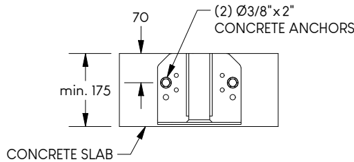
CONCRETE APPLICATION
