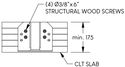
WOOD APPLICATION
