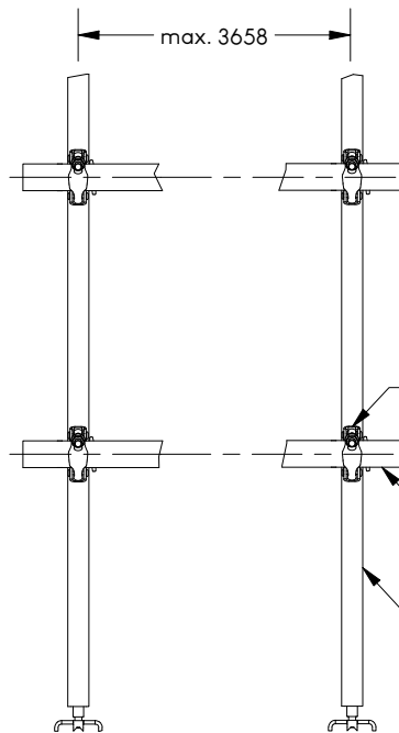
APPLICATION DETAILS (FRONT ELEVATION)
